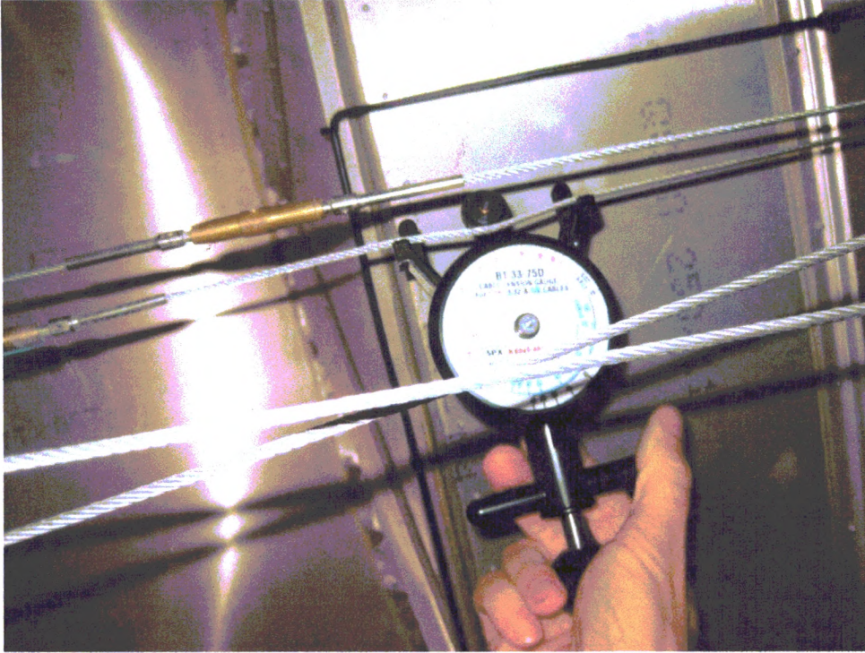
Above: Checking elevator cable tension inside fuselage.
