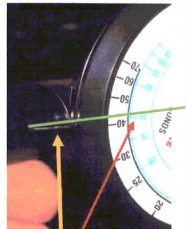
Index mark (read blue scale for 1/8 cables)
