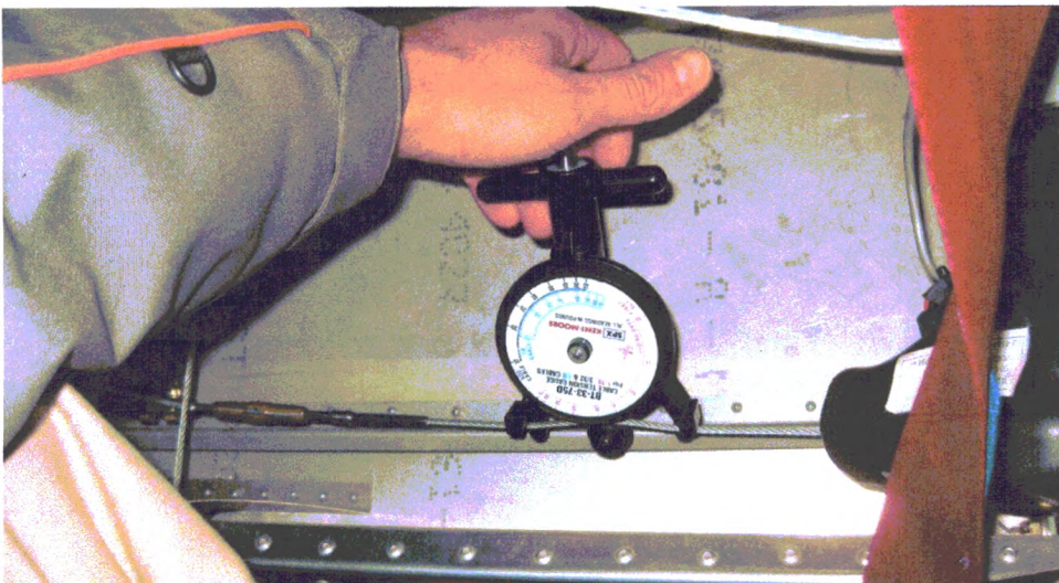
Photo of tensiometer on left Aileron cable seen from pilot seat (see flap motor on right). Repeat process on right aileron cable, behind passenger seat.
